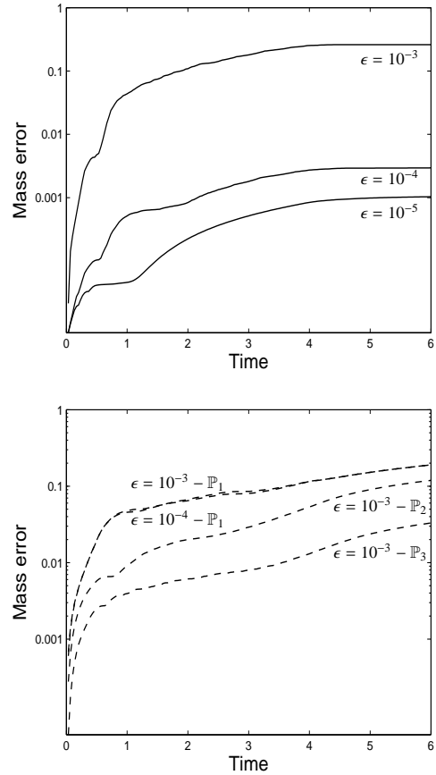
Figure 12: TC3 - Mass error for DDFV (solid lines) and SWIP (dashed lines).
